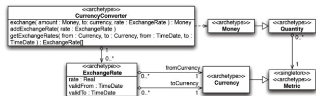
Figure 6. CurrencyConverter archetype
