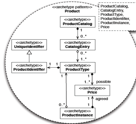
Figure 2. Parameterised collaboration [11]
