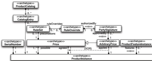
Figure 7. UniqueProduct pleomorph [11]
